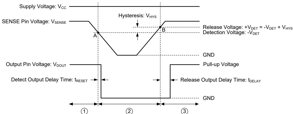
Figure 8. SGM880E-xQ Diagram
