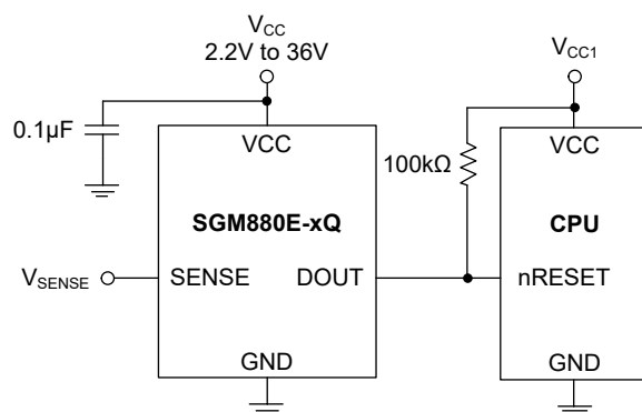
Figure 18. SGM880E-xQ Typical Application Circuit
