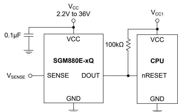
Figure 2. SGM880E-xQ Typical Application Circuit
