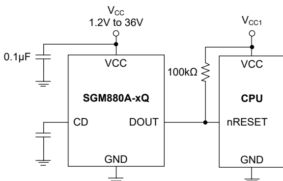
Figure 1. SGM880A-xQ Typical Application Circuit
