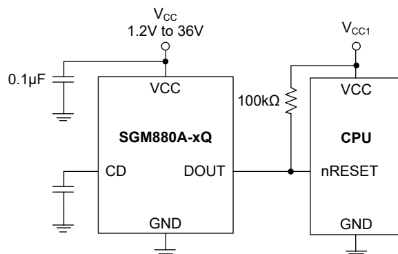
Figure 17. SGM880A-xQ Typical Application Circuit
