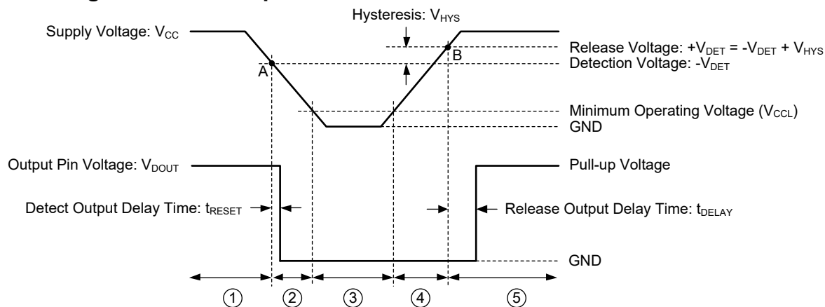
Figure 7. SGM880A-xQ Diagram
