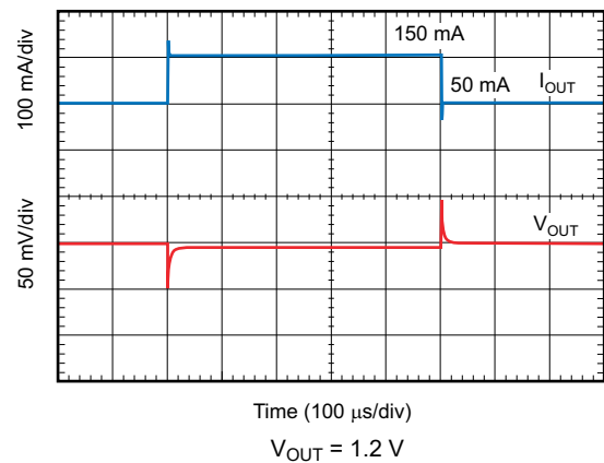
图 6-40. Load Transient Response
