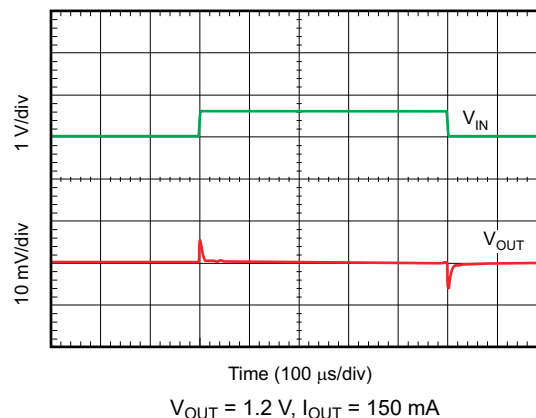
图 8-5. Line Transient Response
