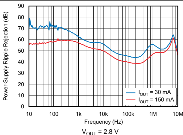
图 6-33. Power-Supply Ripple Rejection vs Frequency
