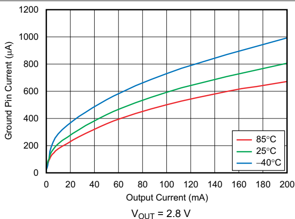
图 6-24. Ground Pin Current vs Output Current
