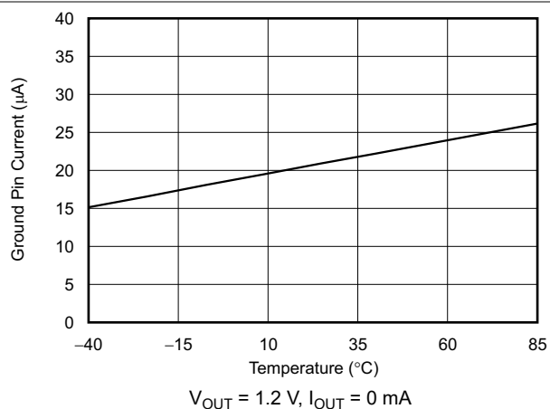
图 6-20. Ground Pin Current vs Temperature
