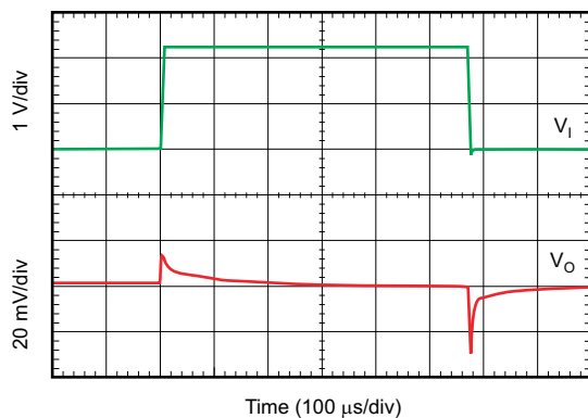
图 6-51. Line Transient Response
