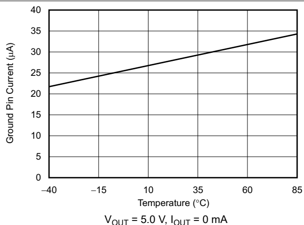
图 6-22. Ground Pin Current vs Temperature
