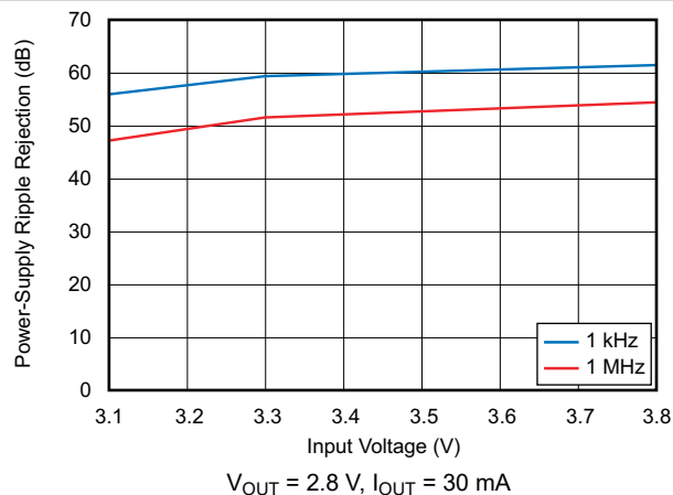
图 6-35. Power-Supply Ripple Rejection vs Input Voltage
