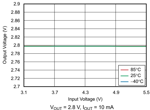
图 6-5. Line Regulation
