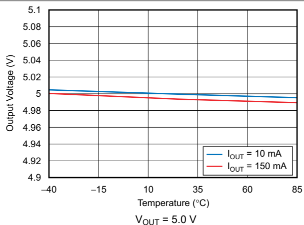
图 6-12. Output Voltage vs Temperature
