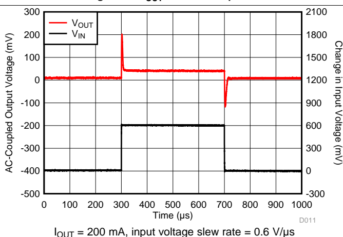
Figure 18. V_{IN} Transient
