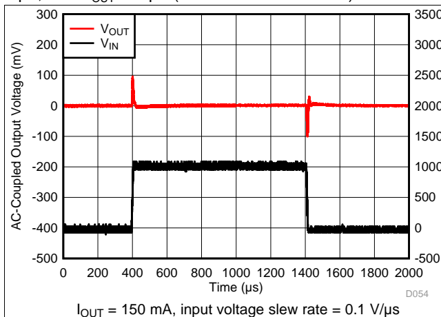
Figure 19. V_{IN} Transient
