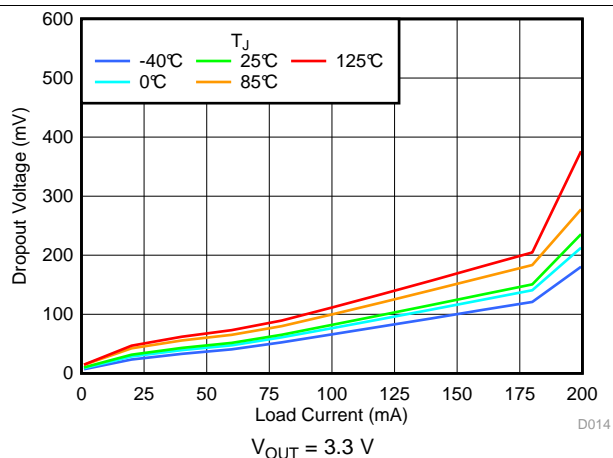
Figure 22. Dropout vs I_{OUT} and Temperature
