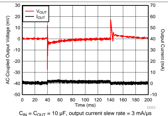
Figure 16. I_{OUT} Transient 3 \mu\text{A} to 3 mA
