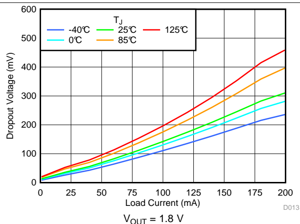
Figure 21. Dropout vs I_{OUT} and Temperature
