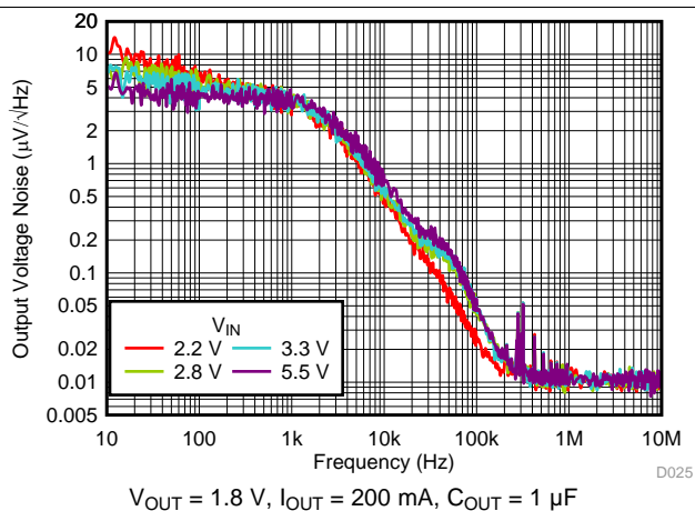
Figure 42. Output Noise vs Frequency and V_{IN}
