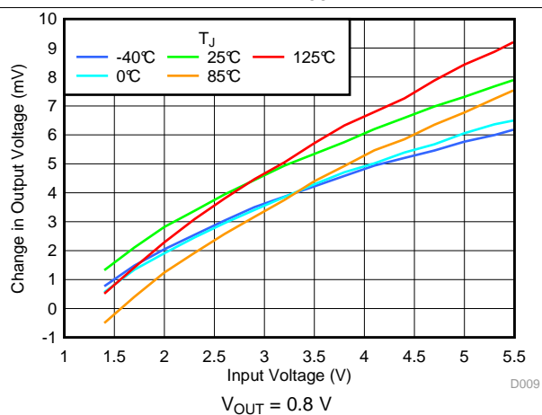
Figure 24. Line Regulation V_{IN} and Temperature
