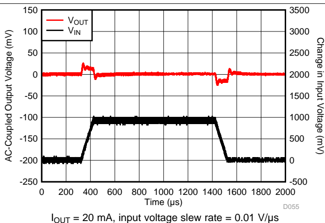
Figure 20. V_{IN} Transient
