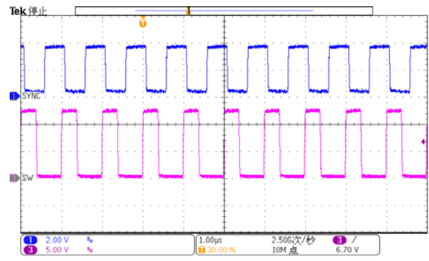
Figure 24. Sync Frequency
