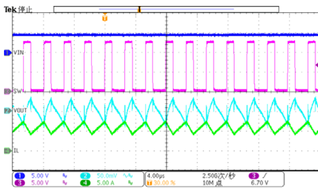
Figure 23. Steady-state (Iload=2A)
