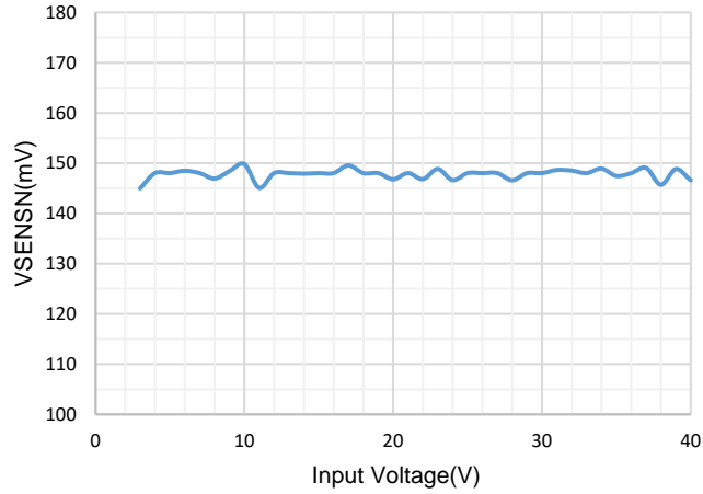
Figure 7. VSENSEN vs Input Voltage
