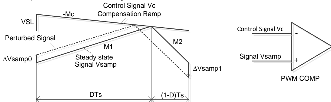
Figure12. Sub-Harmonic Oscillation for D > 0.5 and Compensation Ramp to Avoid Sub-Harmonic Oscillation
