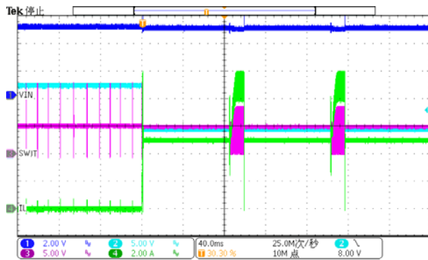
Figure 21. Over current protection (Iload=5A)
