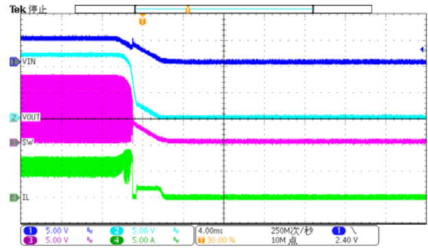
Figure 20. Power down(Iload=2A)
