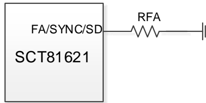
Figure14. Frequency Adjust
