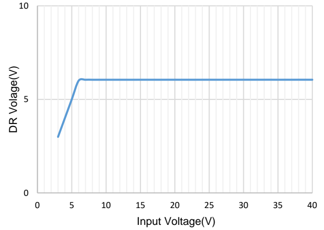
Figure 8. DR Voltage vs Input Voltage
