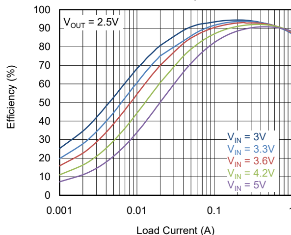
SGM6029C PWM Efficiency vs. Load Current
