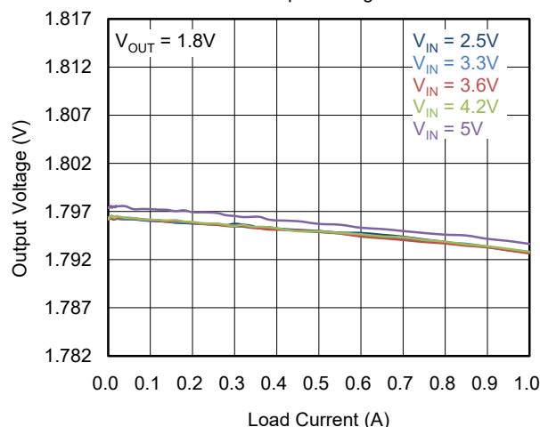
SGM6029C PWM Output Voltage vs. Load Current
