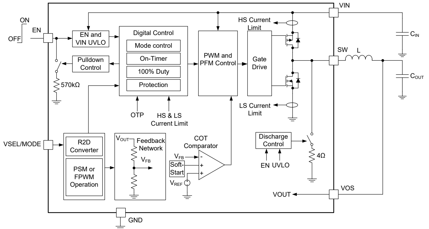
Figure 2. Block Diagram
