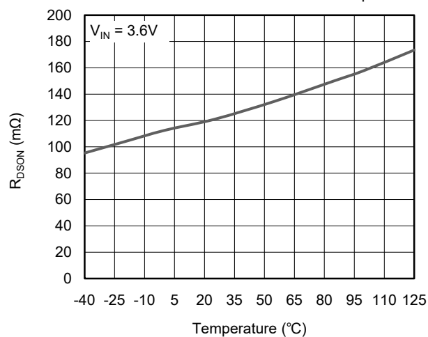
Low-side MOSFET On-Resistance vs. Temperature
