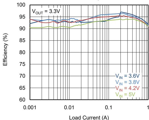
SGM6029C PSM Efficiency vs. Load Current
