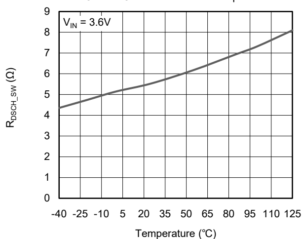
MOSFET On-Resistance vs. Temperature
