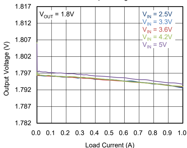
SGM6029C PSM Output Voltage vs. Load Current
