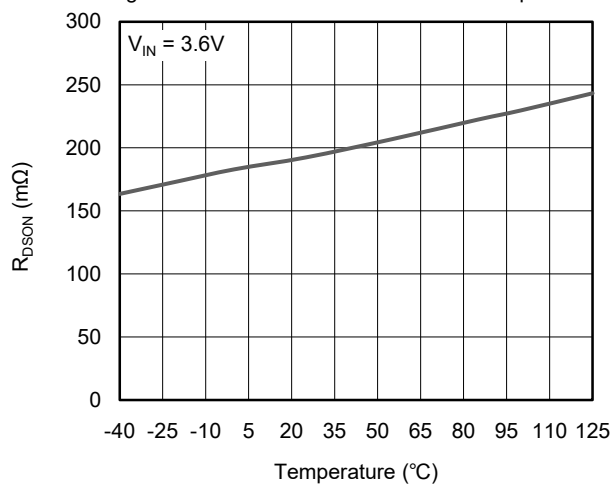
High-side MOSFET On-Resistance vs. Temperature
