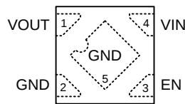
ZQFN-4L 1x1
