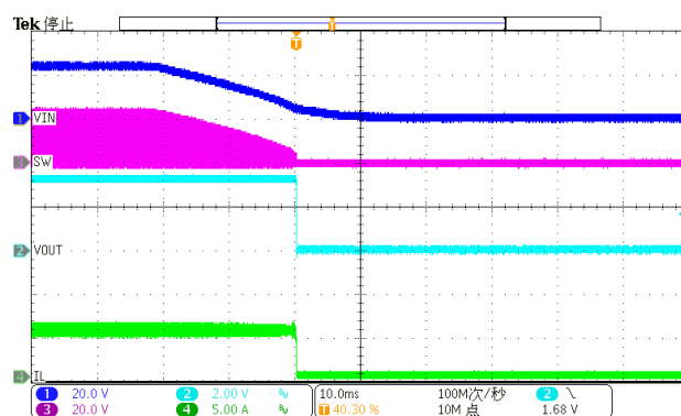
Figure 14. Power down(Iload=5A)
