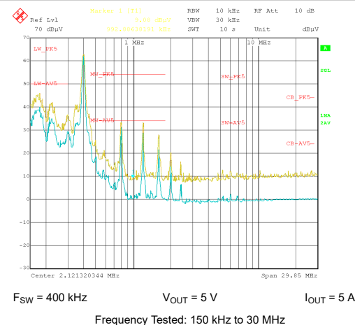
图 10-46. Conducted EMI versus CISPR25 Limits (Yellow: Peak Signal, Blue: Average Signal)
