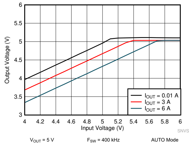
图 10-23. Dropout Curve
