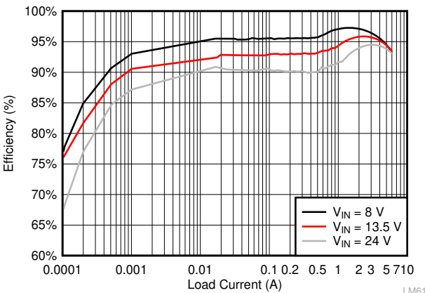
效率：，V OUT = 5V，F SW = 400kHz
