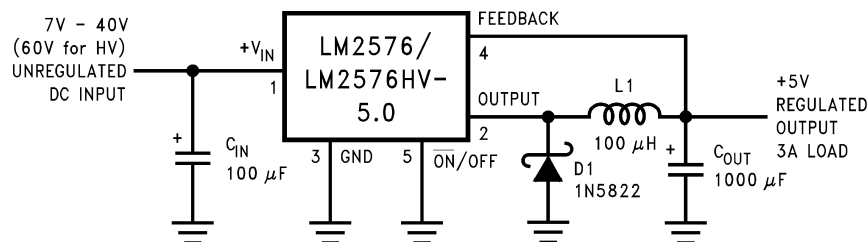
Fixed Output Voltage Version Typical Application Diagram
