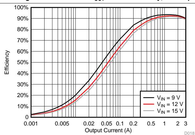
Figure 16. TPS563208 V_{OUT} = 1.8\text{ V} Efficiency, L = 2.2\text{ }\mu\text{H}
