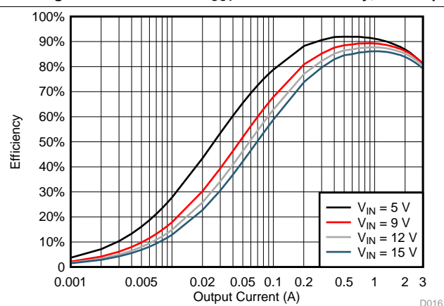
Figure 14. TPS563208 V_{OUT} = 1.05\text{ V} Efficiency, L = 2.2\text{ }\mu\text{H}
