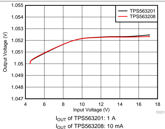
Figure 22. TPS563201 and TPS563208 Line Regulation
