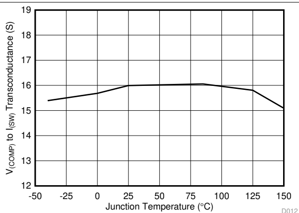
Figure 11. COMP to SW Transconductance vs Junction Temperature
