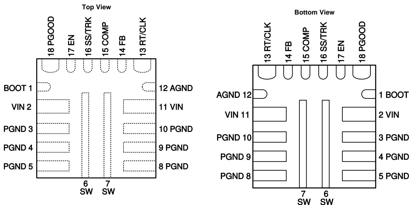
Pin Functions
