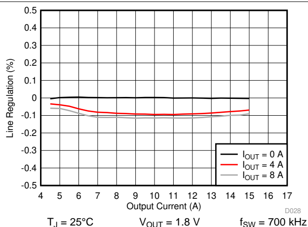
Figure 36. Line Regulation
