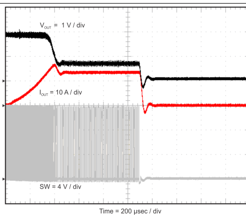
Figure 46. EN Shutdown
