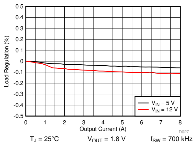
Figure 35. Load Regulation
