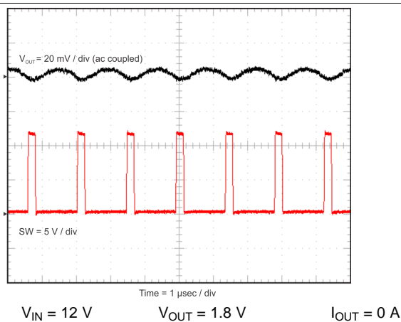
Figure 39. Output Ripple, No Load
