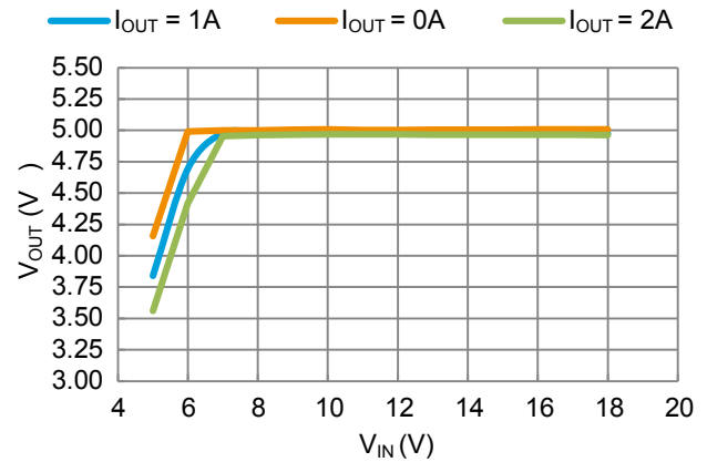
Line Regulation
