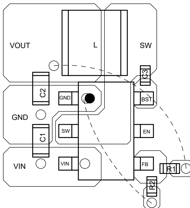
Recommended PCB Layout, TSOT26 Package
