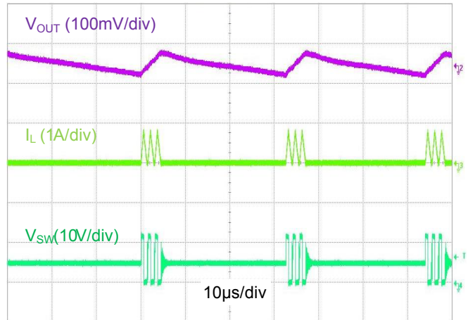
Output Voltage Ripple, V_{OUT} = 5V , I_{OUT} = 50mA
