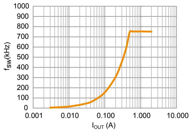
f_{sw} vs. Load
