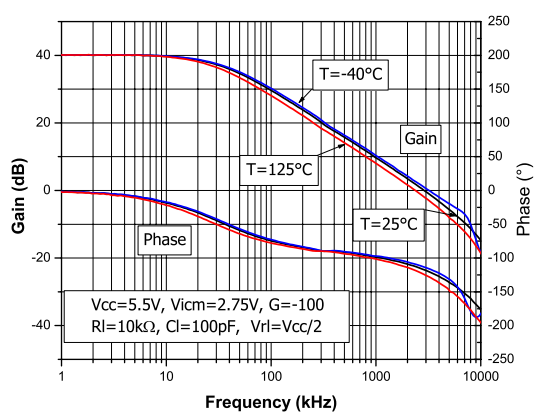
Figure 22. Bode diagram at V_{CC} = 5.5\text{ V}
