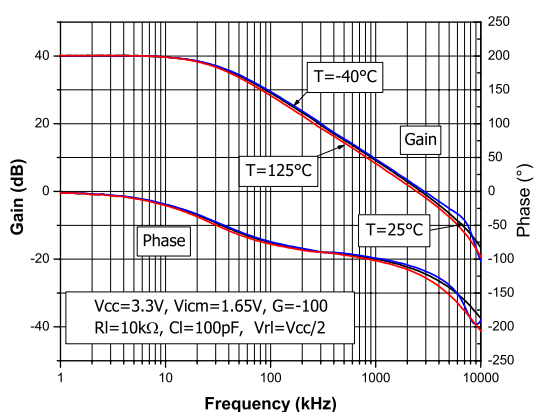
Figure 24. Bode diagram at V_{CC} = 3.3\text{ V}
