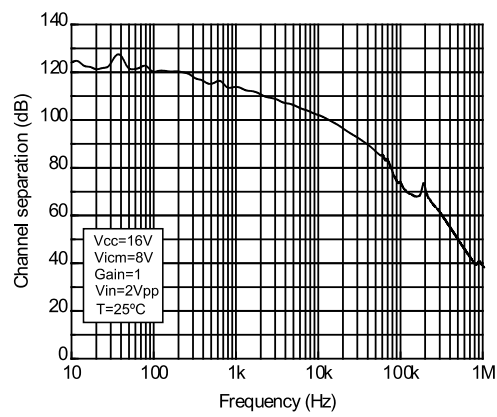
Figure 32: Channel separation (TSX712)
