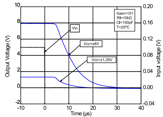
Figure 21: Recovery behavior after a negative step on the input
