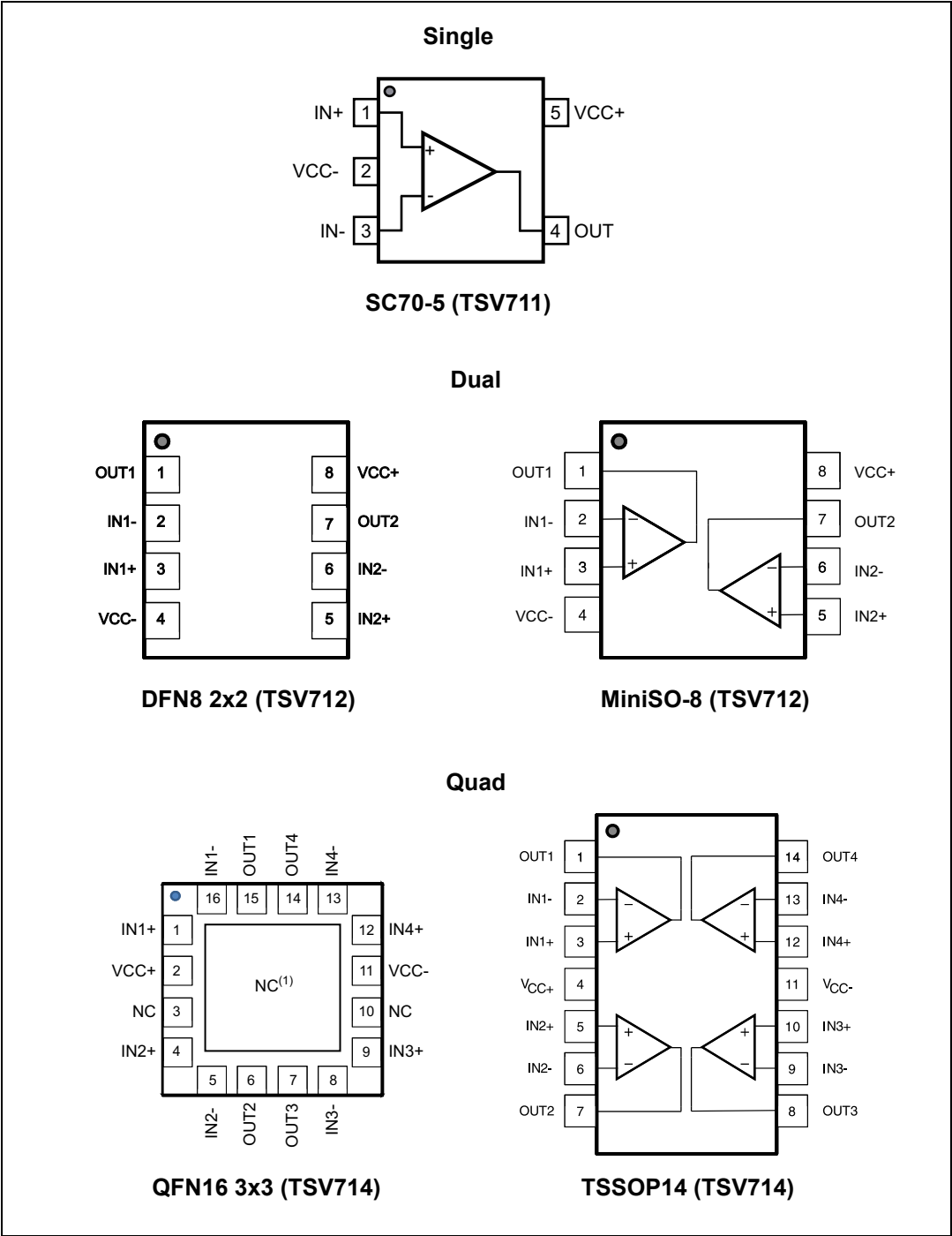
Figure 1. Pin connections (top view)
