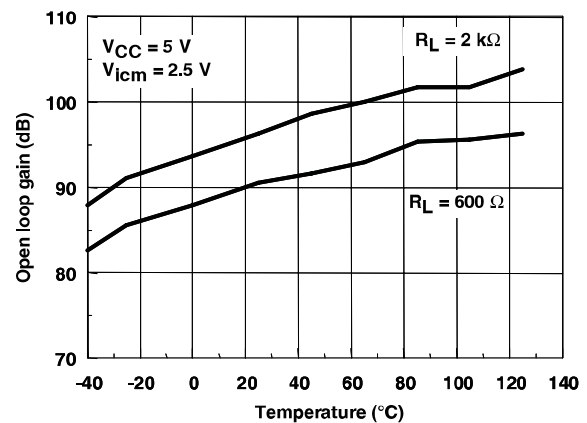
Figure 6: Open loop gain vs. temperature at V_{\text{CC}} = 5\text{ V}
