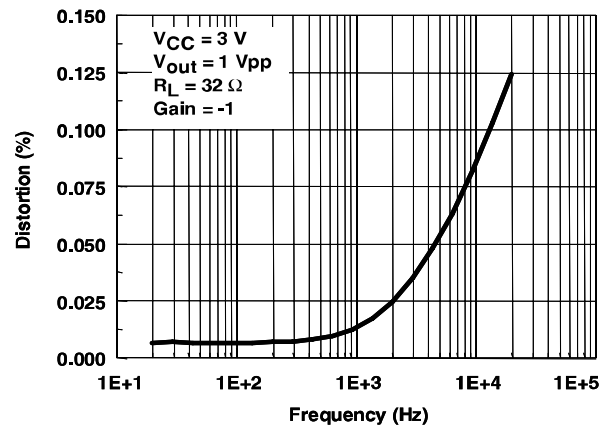
Figure 18: Distortion vs. frequency
