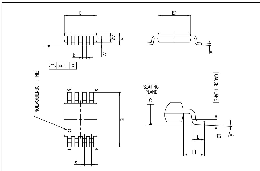
Figure 21: MiniSO8 package outline
