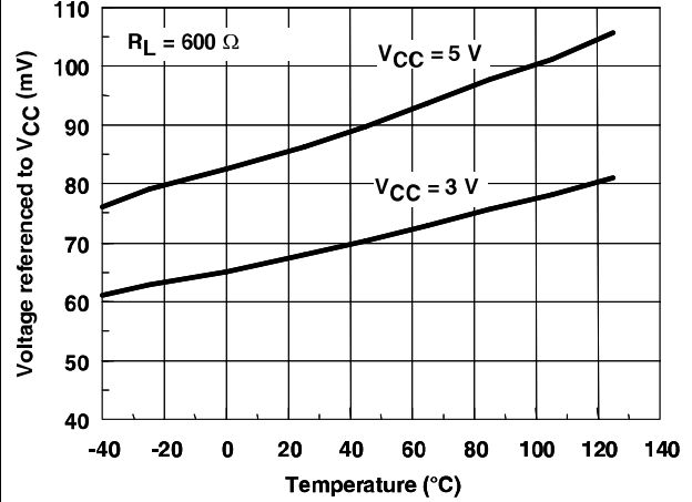
Figure 8: High level output voltage vs. temperature
