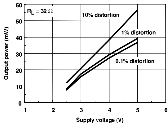
Figure 3: Output power vs. supply voltage
