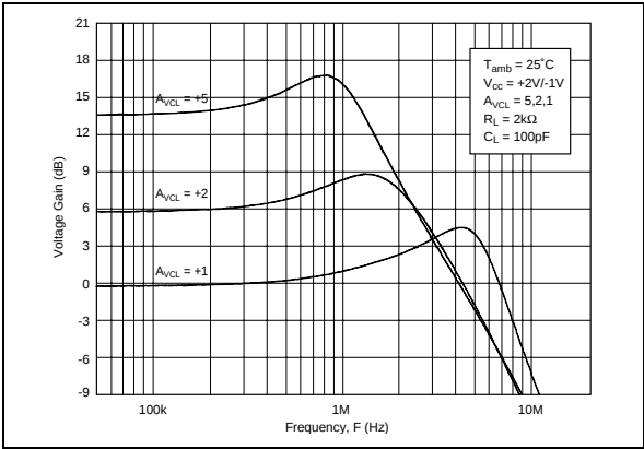
CLOSED LOOP BANDWIDTH @ 3V
