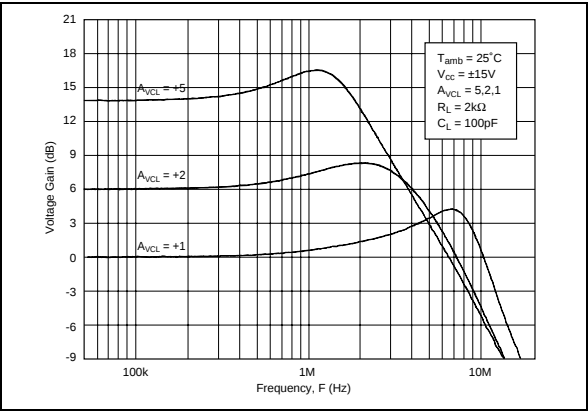
CLOSED LOOP BANDWIDTH @ 30V
