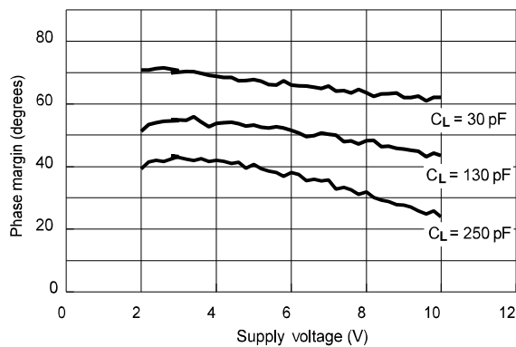
Figure 12: Phase margin vs. VCC CL = 30, 130, and 250 pF
