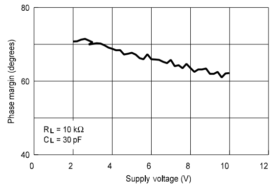
Figure 11: Phase margin vs. VCC RL = 10 kΩ, CL = 30 pF
