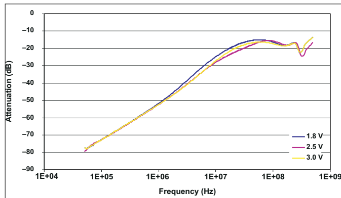
Figure 6-7. OFF Isolation
