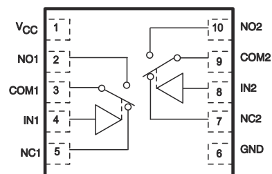
Figure 5-2. DRC Package, 10-Pin VSON (Top View)
