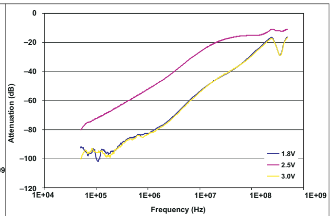
Figure 6-8. Crosstalk
