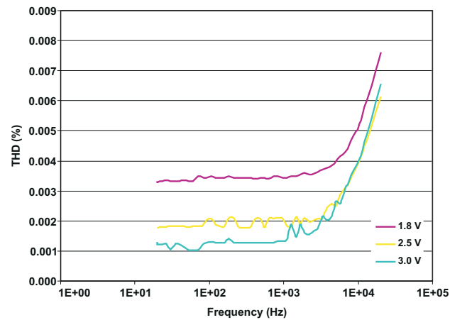
Figure 6-9. Total Harmonic Distortion vs Frequency
