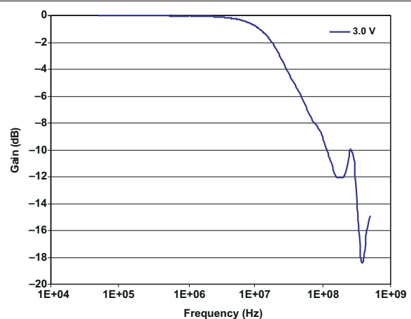
Figure 6-6. Bandwidth
