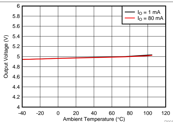
Figure 1. 5-V Output Voltage vs Ambient Temperature
