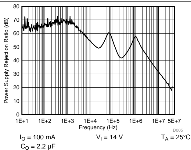
Figure 8. Power Supply Rejection Ratio
