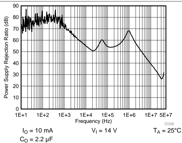
Figure 9. Power Supply Rejection Ratio
