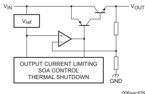
Fig 2. Fixed output voltage versions: functional diagram
