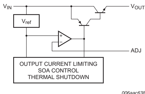
Fig 1. Adjustable output voltage versions: functional diagram
