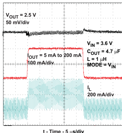
Figure 52. Load Transient Response 5 mA to 200 mA, Forced PWM Mode, V_{OUT} 2.5 V – TPS62230
