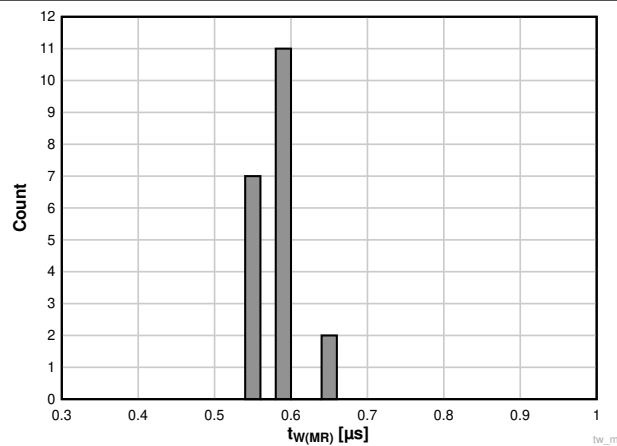
Figure 7-22. Manual Reset Pulse Width Histogram for TPS3823A-33 Devices at 25°C (Unit Count = 20)
