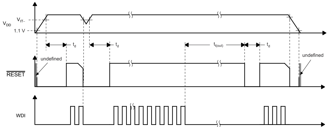
Figure 7-1. Timing Diagram
