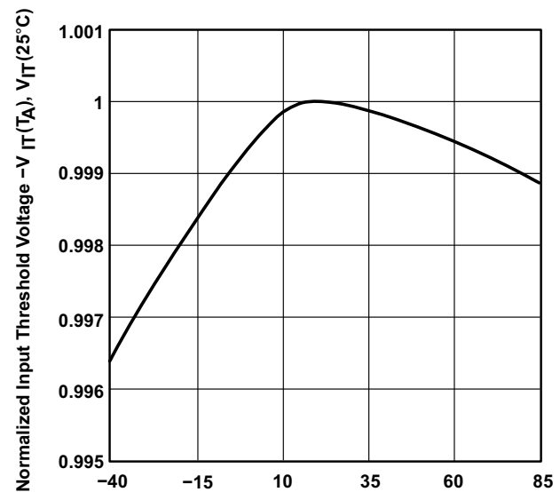
Normalized Input Threshold Voltage vs Free-Air Temperature
