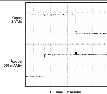
Figure 65. 2-Ω Load Connected to Enabled Device
