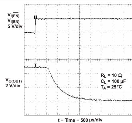
Figure 37. Turnoff Delay and Fall Time With 100-μF Load
