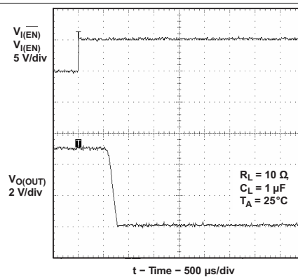
Figure 20. Turnoff Delay and Fall Time With 1-μF Load
