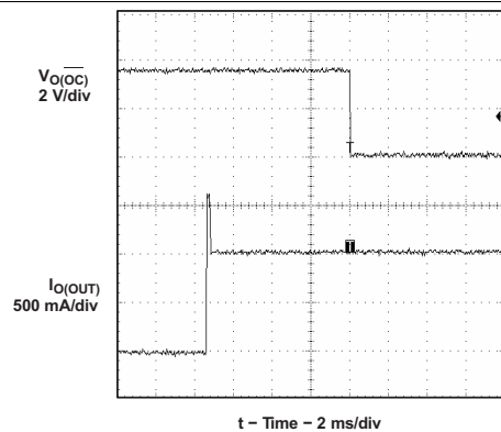
Figure 64. 3-Ω Load Connected to Enabled Device
