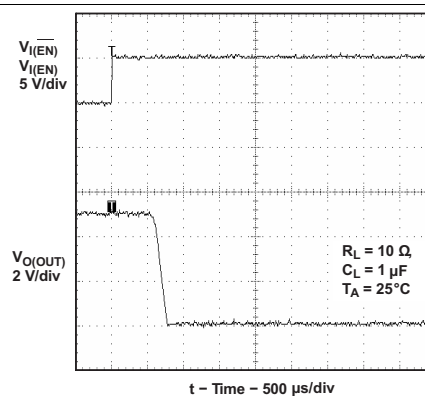
Figure 59. Turnoff Delay and Fall Time With 1-μF Load
