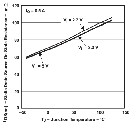
Figure 13. Static Drain-Source on-State Resistance vs Junction Temperature
