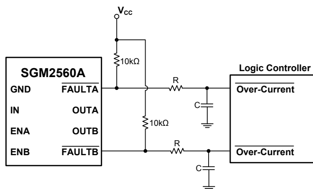
Figure 6. Transient Filter
