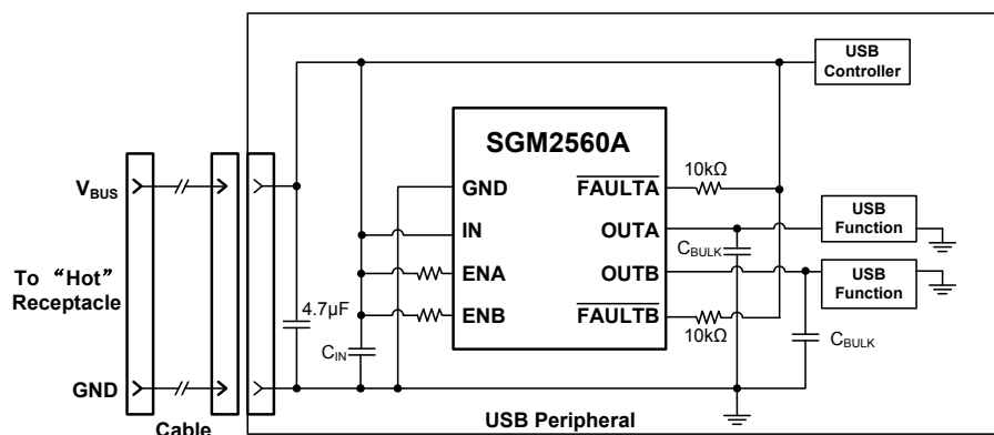
Figure 5. Hot-Plug Application
