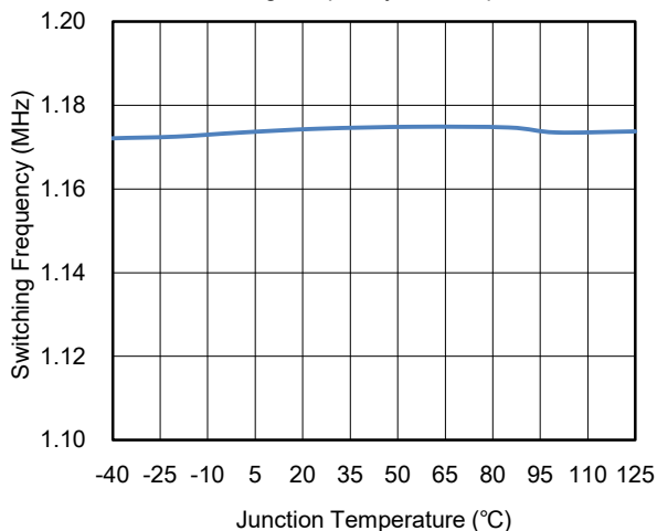
Switching Frequency vs. Temperature
