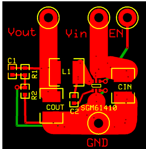
Figure 6. Suggested PCB
