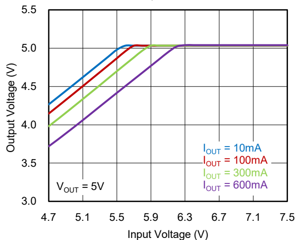
Dropout Curve
