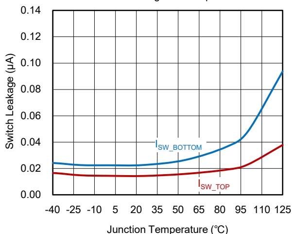
Switch Leakage vs. Temperature
