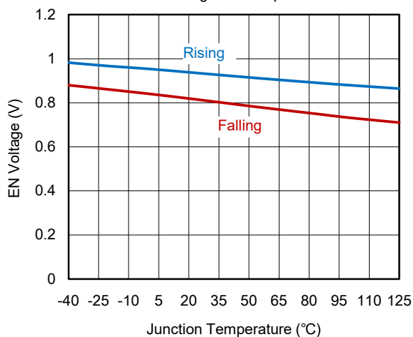
EN Voltage vs. Temperature
