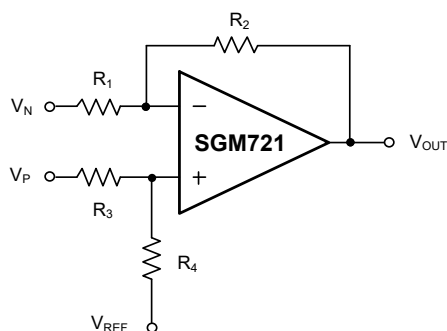
Figure 4. Differential Amplifier
