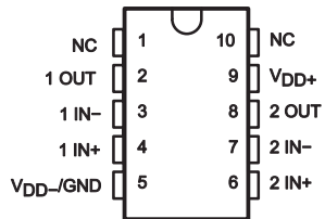
TLC2272 U Package 10-Pin CFP Top View
