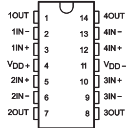
TLC2274 D, J, N, PW, or W Package 14-Pin SOIC, CDIP, PDIP, TSSOP, or CFP Top View
