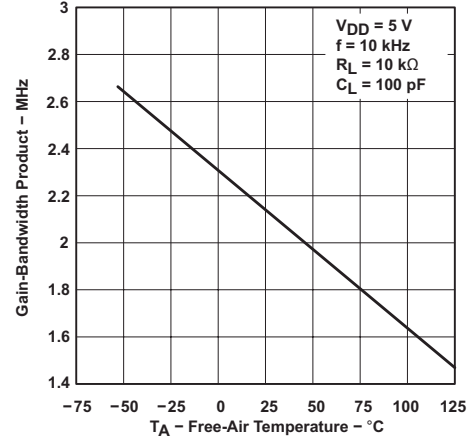
Figure 56. Gain-Bandwidth Product vs Free-Air Temperature
