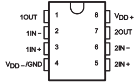
TLC2272 D, JG, P, or PW Package 8-Pin SOIC, CDIP, PDIP, or TSSOP Top View
