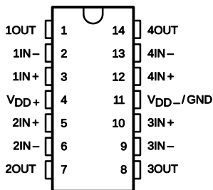
TLC2264C, TLC2264AC TLC2264I, TLC2264AI TLC2264Q, TLC2264AQ D, N, OR PW PACKAGE (TOP VIEW)
