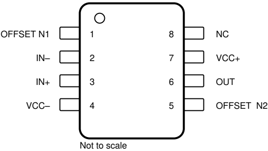
Figure 5-4. TL071x D, P, and PS Package 8-Pin SOIC, PDIP, and SO (Top View)
