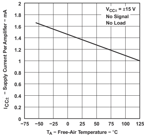
Figure 6-52. Supply Current Per Amplifier vs Free-Air Temperature
