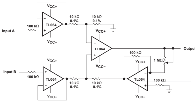
Figure 21. Instrumentation Amplifier
