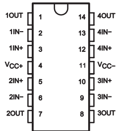
TL064x D, J, N, NS, PW, and W Package 14-Pin SOIC, CDIP, PDIP, SO, TSSOP and CFP Top View
