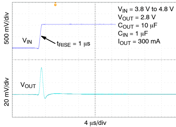
Figure 35. Line Transient Response – Rising Edge, V_{OUT} = 2.8 \text{ V} , I_{OUT} = 300 \text{ mA}
