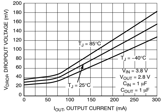
Figure 12. Dropout Voltage vs. Output Current V_{OUT} = 2.8 \text{ V (UDFN)}
