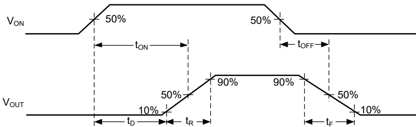
Figure 3. Timing Waveforms
