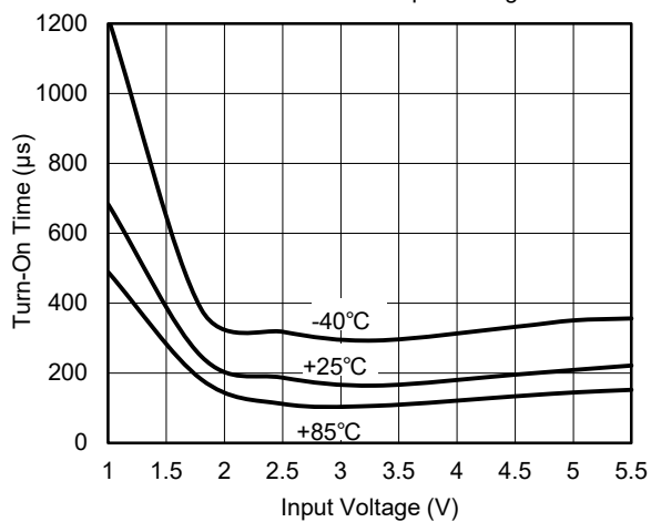
Turn-On Time vs. Input Voltage
