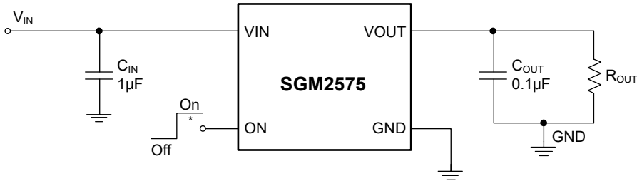
Figure 2. Test Circuit
