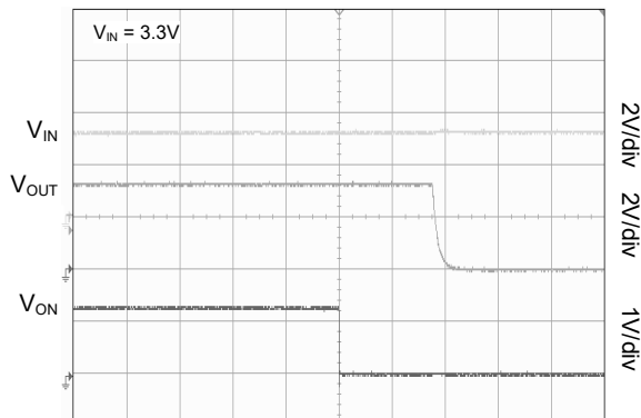
Turn-Off Response
