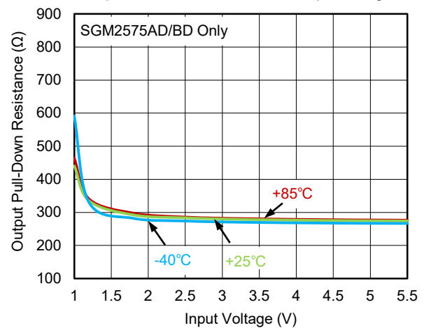
Output Pull-Down Resistance vs. Input Voltage
