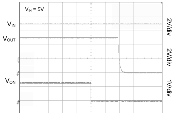
Turn-Off Response
