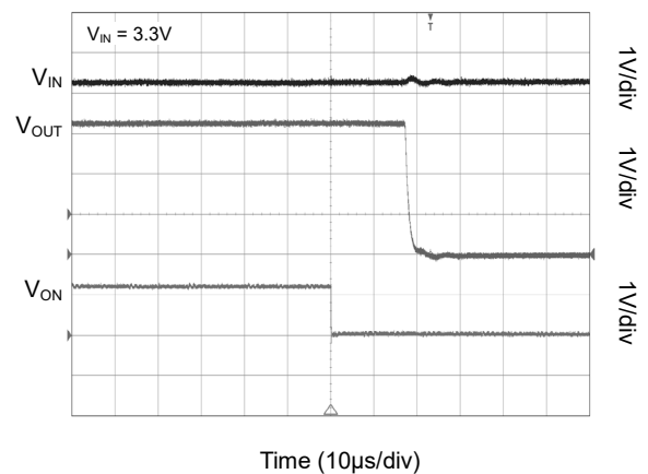
Turn-Off Response
