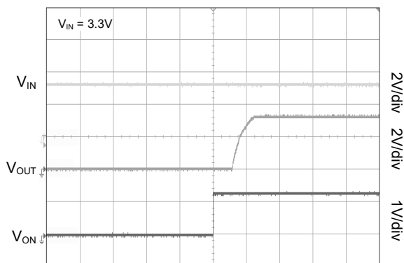
Turn-On Response
