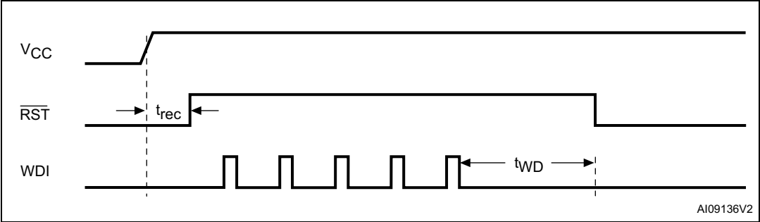
Figure 26. Watchdog timing
