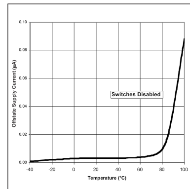
Fig. 9: Off-state Supply Current vs Temperature
