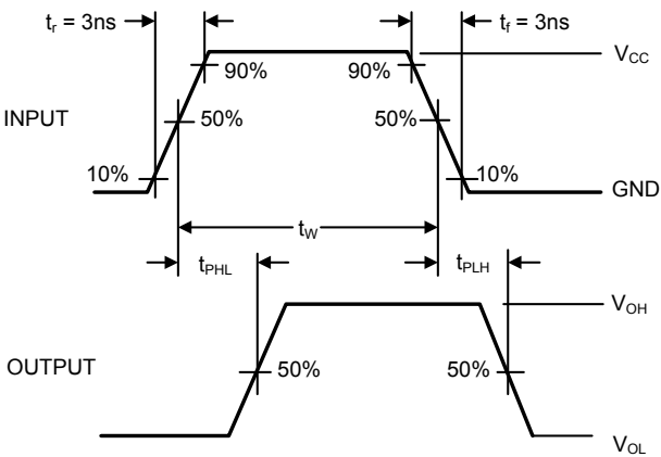
Figure 2. AC Waveforms
