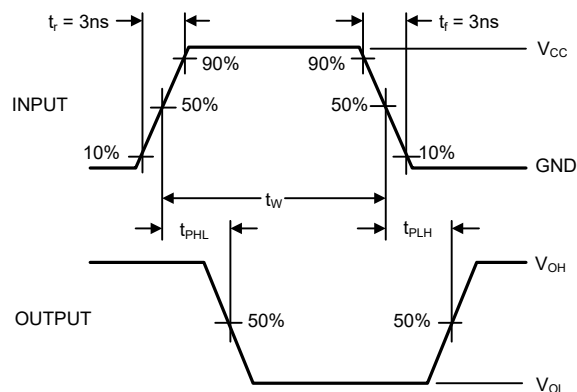
Figure 2. AC Waveforms
