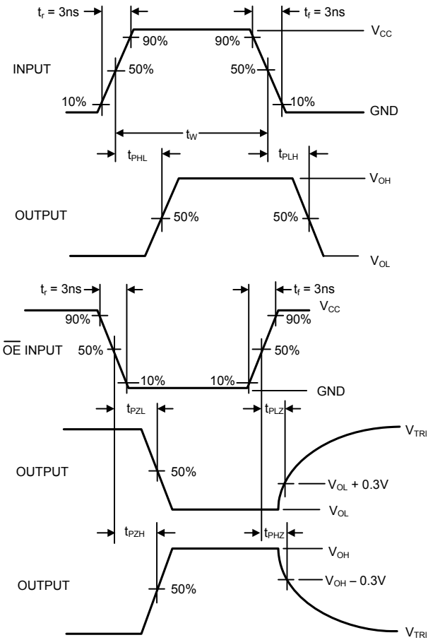
Figure 2. AC Waveforms
