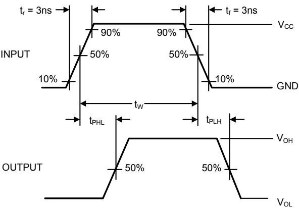
Figure 2. AC Waveforms
