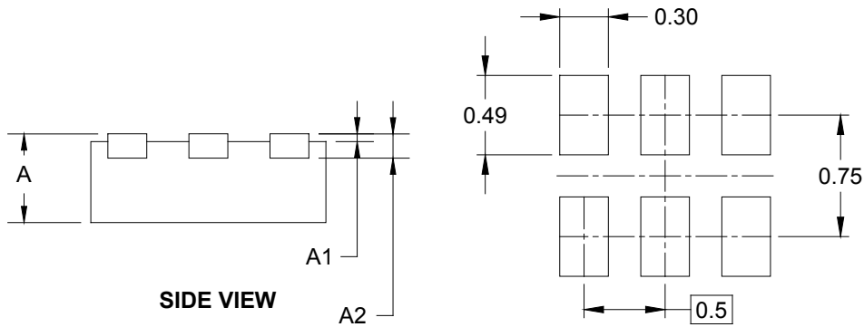
RECOMMENDED LAND PATTERN (Unit: mm)
