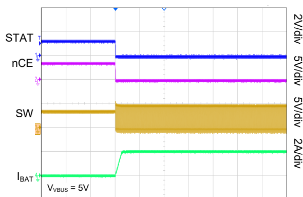
Charge Enable
