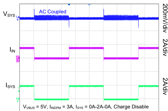
Input Current DPM Response without Battery
