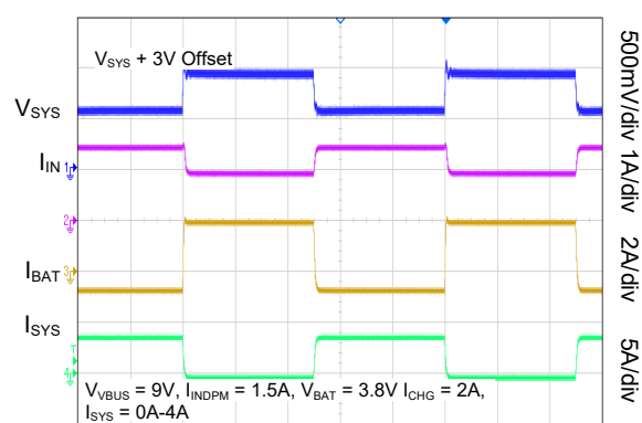
Load Transient during Supplement Mode
