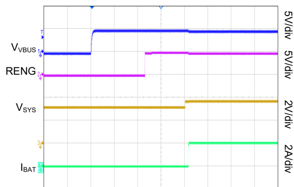
Power-Up with Charge Enabled
