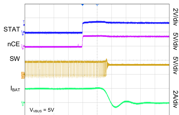
Charge Disable
