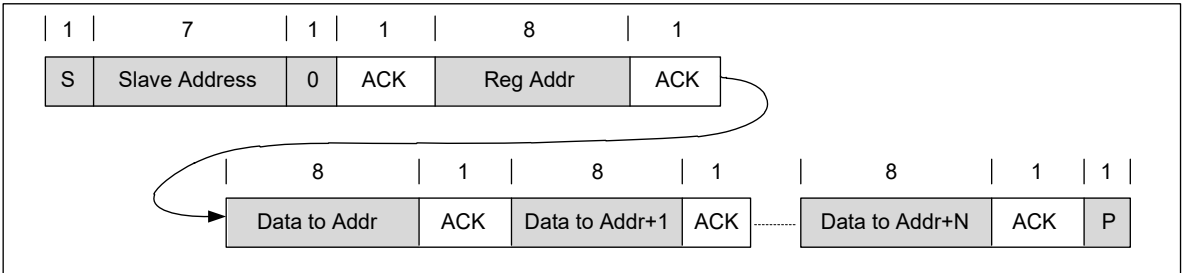
Figure 18. A Multi-Write Transaction
