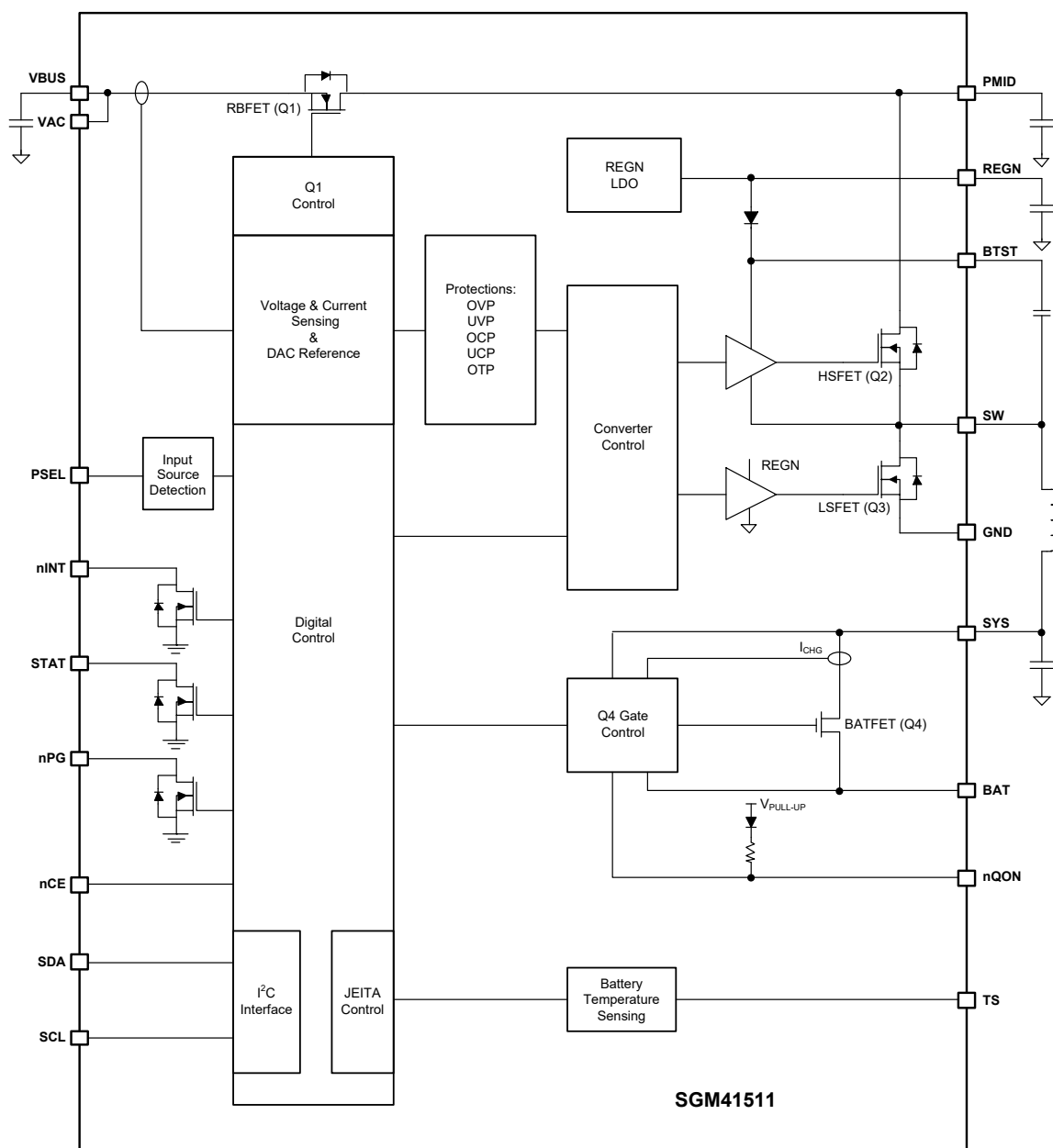
Figure 2. Block Diagram
