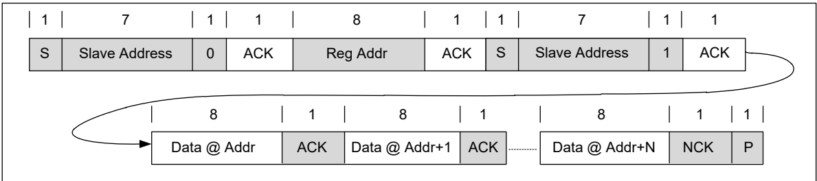
Figure 19. A Multi-Read Transaction
