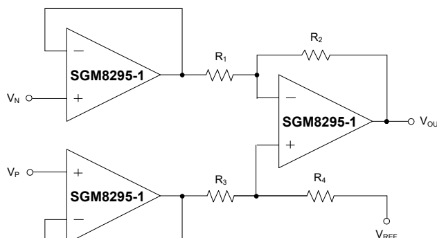
Figure 3. Instrumentation Amplifier
