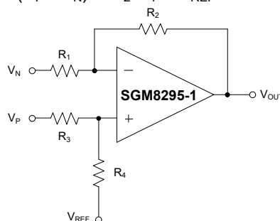
Figure 2. Differential Amplifier
