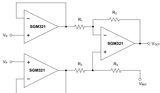
Figure 5. Instrumentation Amplifier
