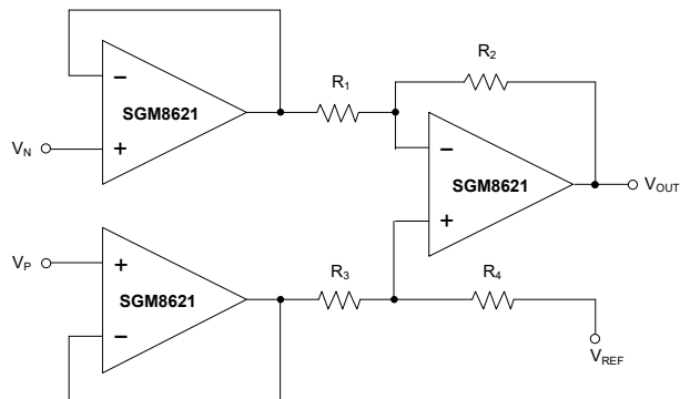
Figure 5. Instrumentation Amplifier
