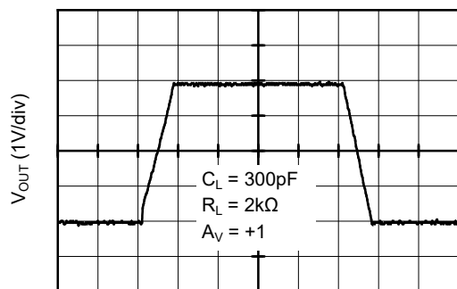
Large Signal Transient Response at +5V
