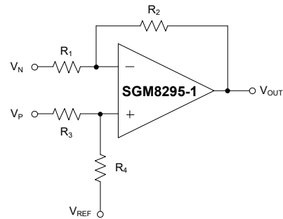
Figure 2. Differential Amplifier
