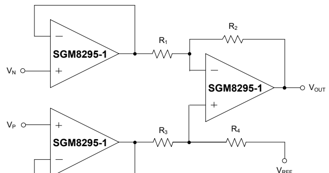
Figure 3. Instrumentation Amplifier
