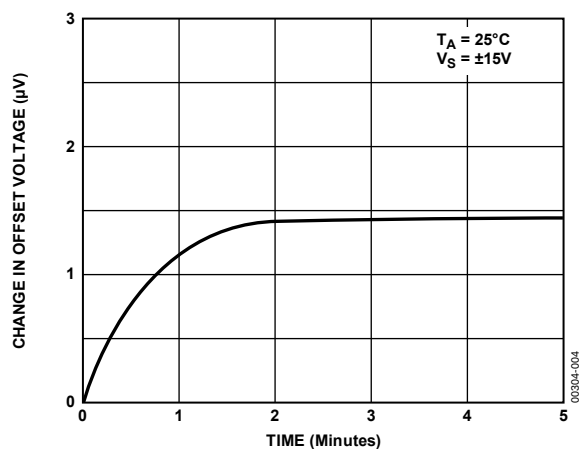
Figure 4. Warmup Drift
