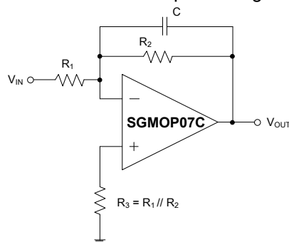
Figure 4. Active Low-Pass Filter
