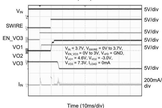
Startup Sequence
