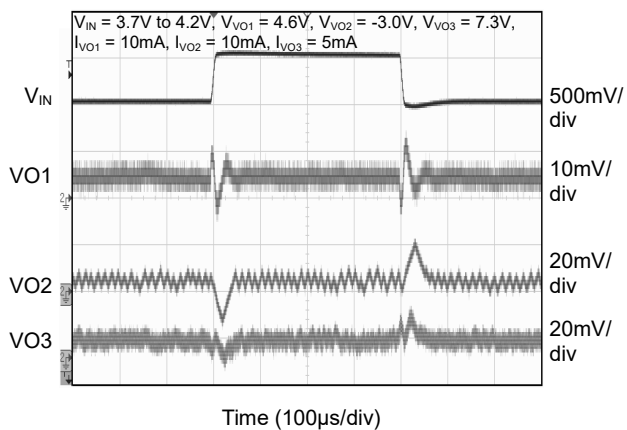
Line Transient at Light Load
