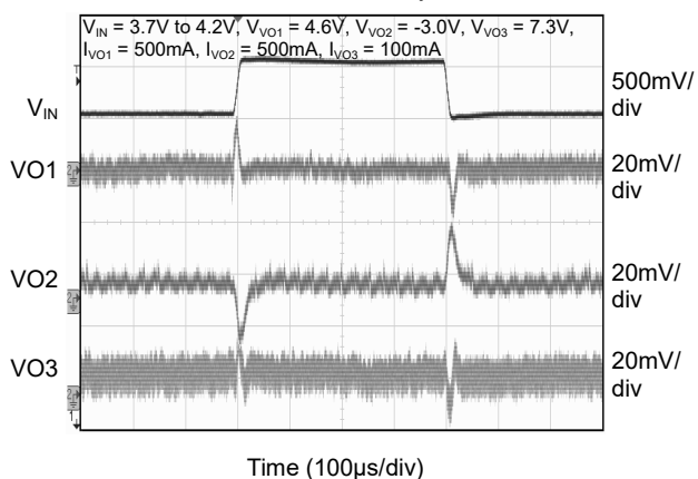
Line Transient at Heavy Load
