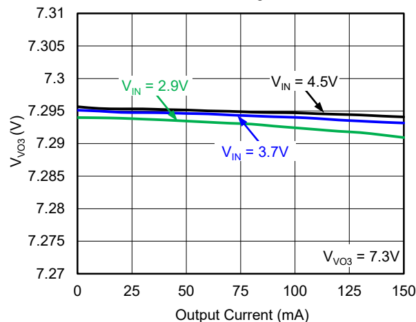
V_{VO3} Load Regulation
